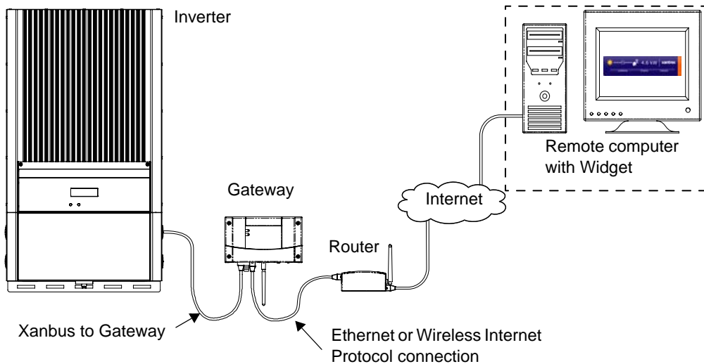
Figure 1-9 Gateway with Widget and Remote Access
