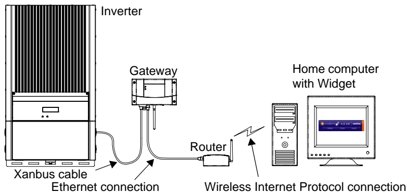
Figure 1-5 Mixed Wired/Wireless Network 2
